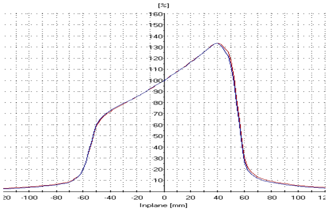
Graphics 5. For 6 MV photon, 45^\circ VV profile in 10x10 cm field; red line for siemens primus, blue line for siemens artiste linac
