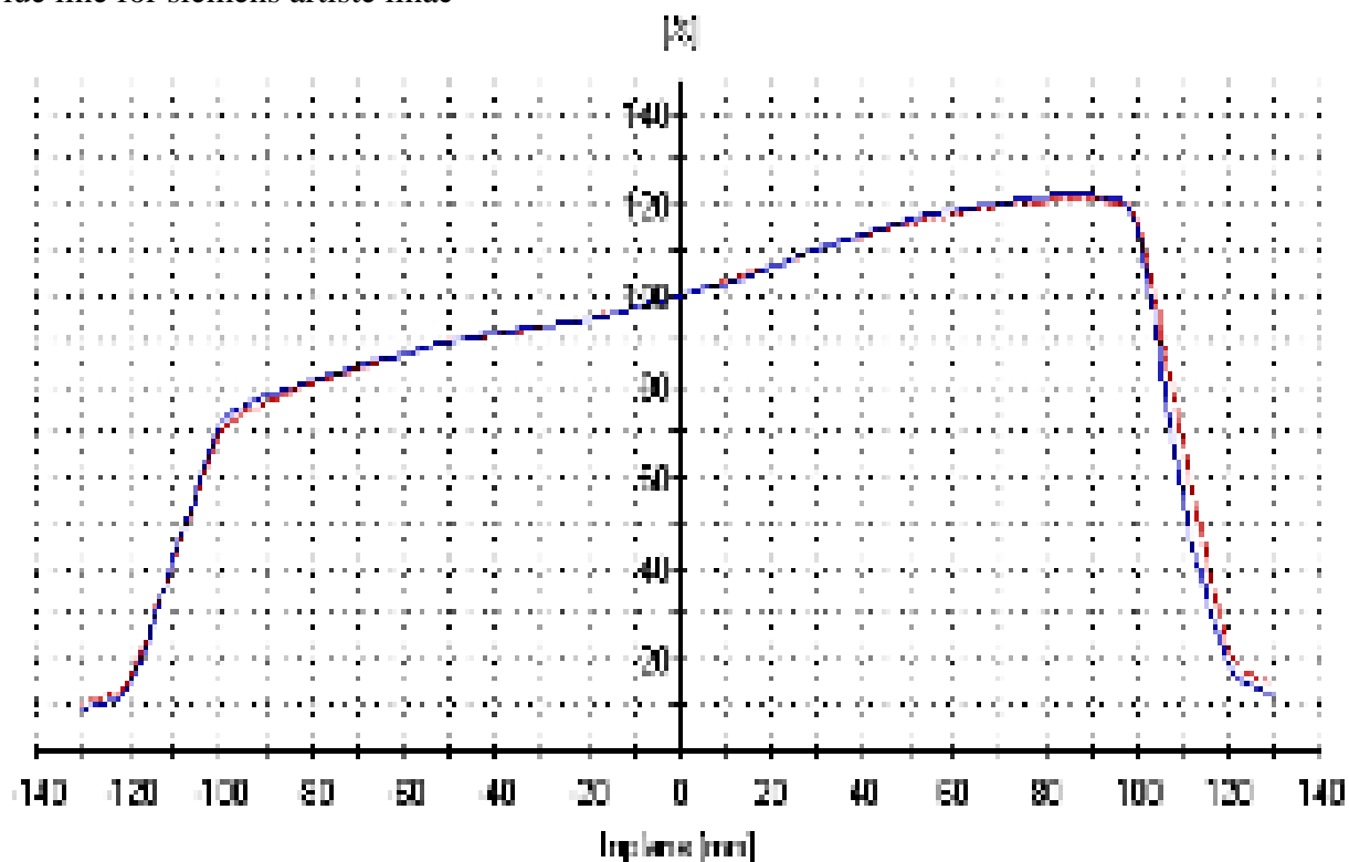
Graphics 4. For 6 MV photon, 30° VW profile in 20x20 cm field; red line for siemens primus, blue line for siemens artiste linac
